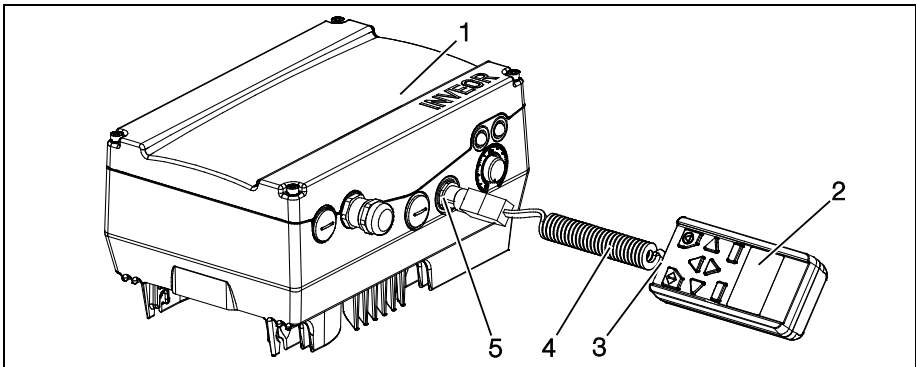
Fig. 3 MMI with EASYdrive drive control
